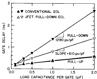
Fig. 10. Simulated delay versus load capacitance at 1 mW/gate for the JFET pull-down ECL circuit and the conventional ECL circuit (FI = FO = 3).
