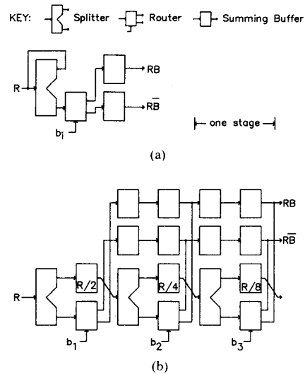
Fig. 1. Block diagram of programmable gain control circuit. (a) Serial recursive circuit. (b) Pipeline circuit.
