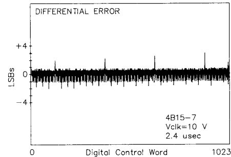
Fig. 4. Differential linearity error of pipeline circuit. Note that the 1-LSB tic mark corresponds to 1/1024 th of full scale.
