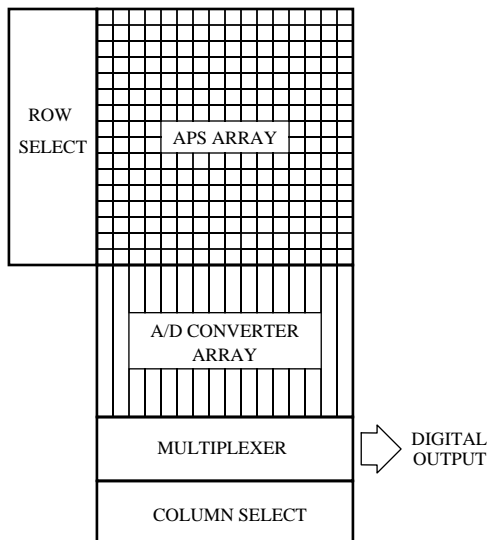
Figure 1: Semi-parallel architecture for focal plane A/D conversion.
