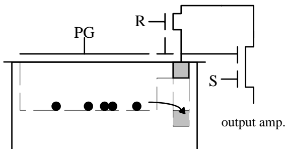
Fig. 2. Schematic illustration of a lateral APS pixel.
