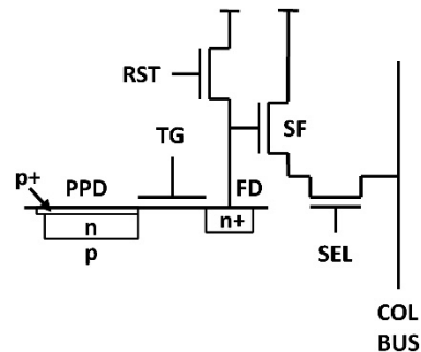
Figure 8. Circuit schematic of CMOS image sensor pixel including reset gate (RST), source-follower (SF), and row select switch (SEL).
