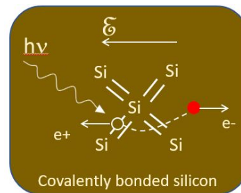
Figure 2. A photon with energy h\nu breaks a silicon bond and frees both an electron ( e^- ) and a hole ( e^+ ).
